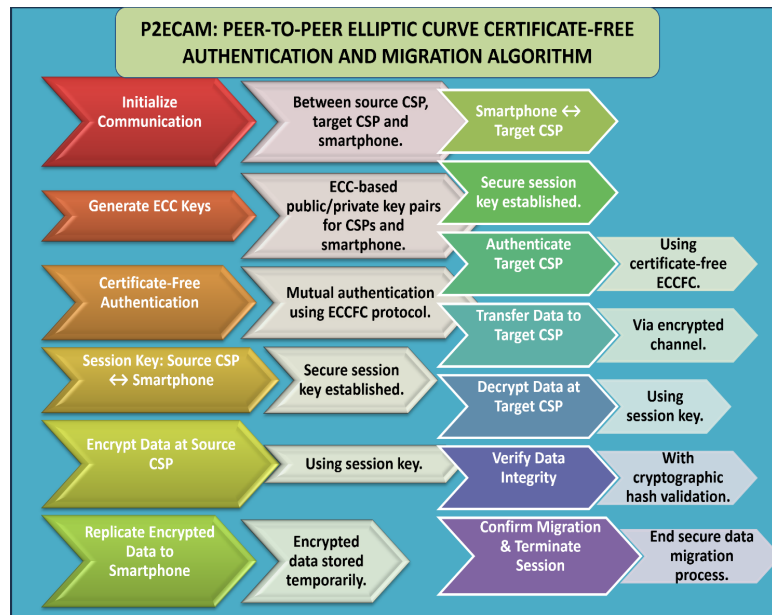
Figure 1: P2ECAM: Peer to peer ECC Authentication and migration Algorithm
