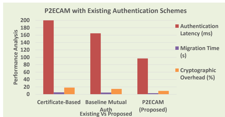
Graph 1: Comparative Performance Analysis of P2ECAM with Existing Authentication Schemes
