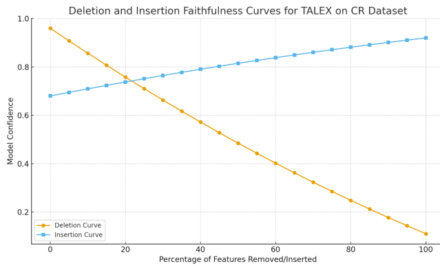
Figure 6: Deletion and insertion faithfulness curves for TALEX on CR dataset
