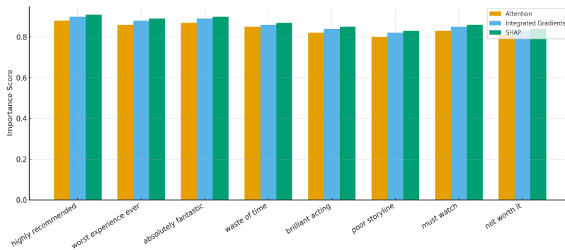
Figure 10: XAI alignment visualization (Attention, IG, SHAP) on IMDB dataset.
