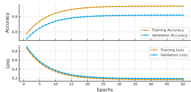
Figure 11: Training and validation accuracy/loss curves for TALEX on SemEval 2013 dataset
