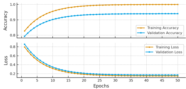
Figure 8: Training and validation accuracy/loss curves for TALEX on IMDB dataset.
