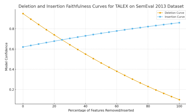
Figure 12: Deletion and insertion faithfulness curves for TALEX on SemEval 2013 dataset.
