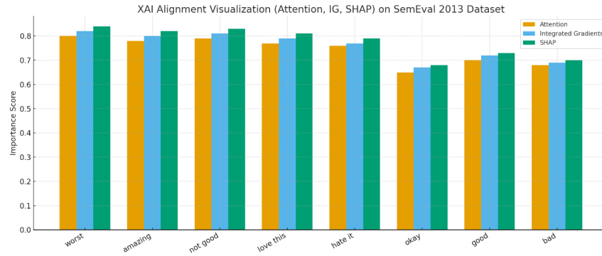
Figure 13: XAI alignment visualization (Attention, IG, SHAP) on SemEval 2013 dataset
