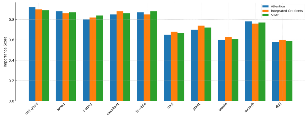
Figure 4: XAI alignment visualization (Attention, IG, SHAP) on MR dataset.
