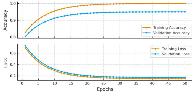
Figure 5: Training and validation accuracy/loss curves for TALEX on CR dataset
