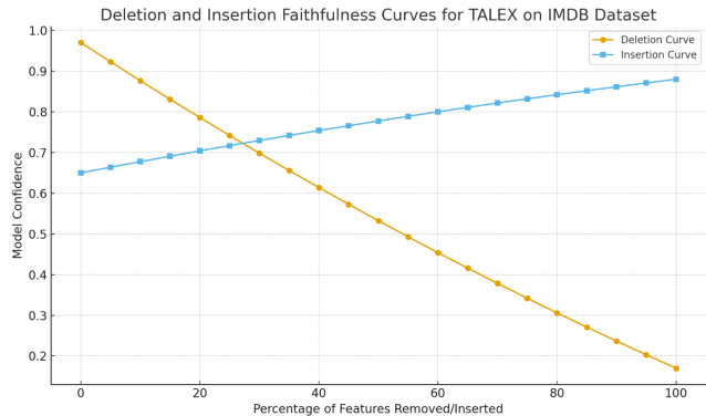
Figure 9: Deletion and insertion faithfulness curves for TALEX on IMDB dataset.
