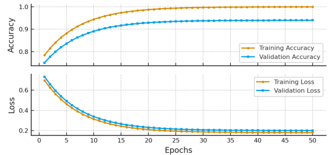
Figure 2: Training and validation accuracy/loss curves for TALEX on MR dataset
