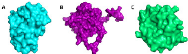
Fig 2: Optimized crystal structures of the target proteins Bak, Bax and Bcl2 from the protein databank database
