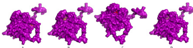
Fig 4: Bax protein with A) DL-norleucine B) 1-tyrosine butyl ester C) Arachidonic acid D) octadecenoic acid
