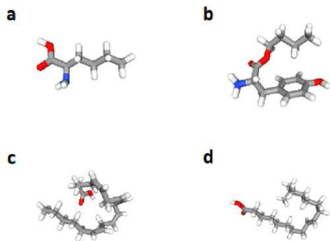
Fig 1: 3D conformers of the ligand compounds retrieved from Pubchem database
