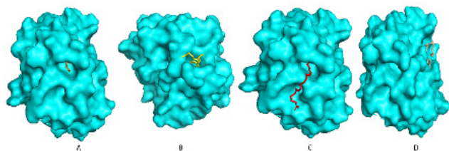
Fig 3: Bax protein with A) DL-norleucine B) 1-tyrosine butyl ester C) Arachidonic acid D) octadecenoic acid
