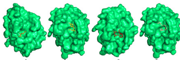
Fig 5: BCL2 protein with A) DL-norleucine B) 1-tyrosine butyl ester C) Arachidonic acid D) Octadecenoic acid
