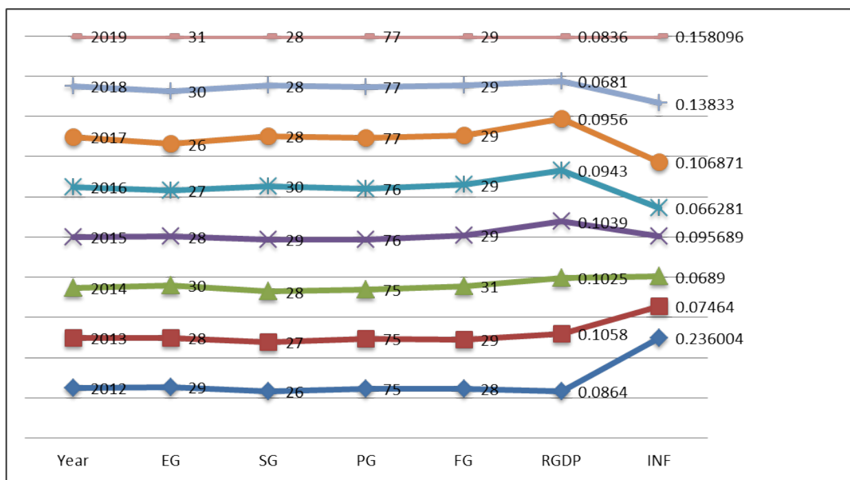
Figure 2: Trend analyses
