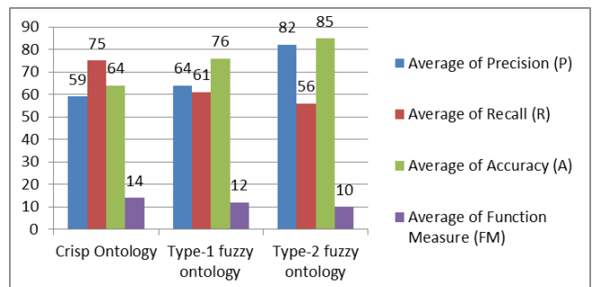
Figure 4: A graphical representation of crisp, type-1, and type-2 fuzzy ontology performance
