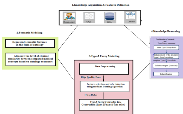
Figure 1: Semantically Intelligent Type-2 fuzzy CDSS System
